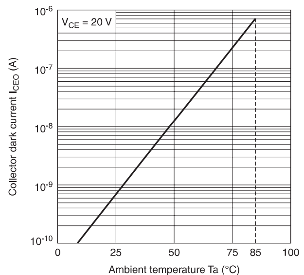
Fig. 2 Collector Dark Current vs. Ambient Temperature
